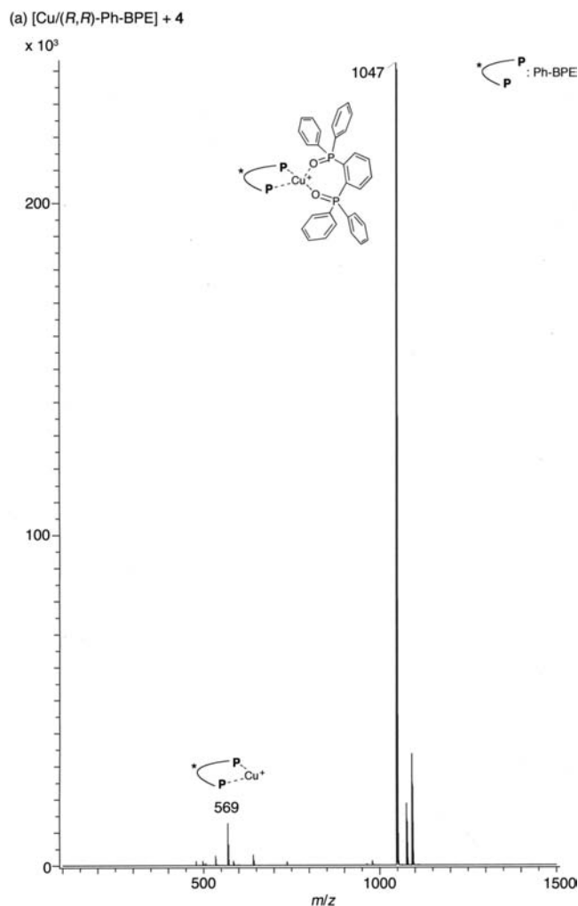
Figure 5. ESI-MS analysis of the solution containing [Cu(CH 3 CN) 4 ]ClO 4 , ( R,R )-Ph-BPE, and 4 (1:1:1).
